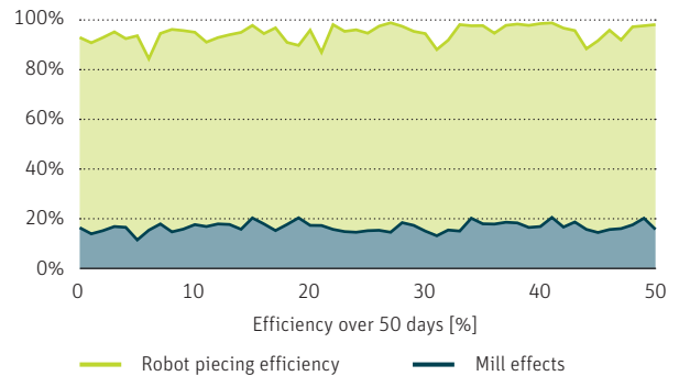
The robot reliably reaches up to 95% piecing efficiency Ne 30, 100% cotton carded G 37 with ISM premium, 18 000 rpm, 1 824 spi/machine
