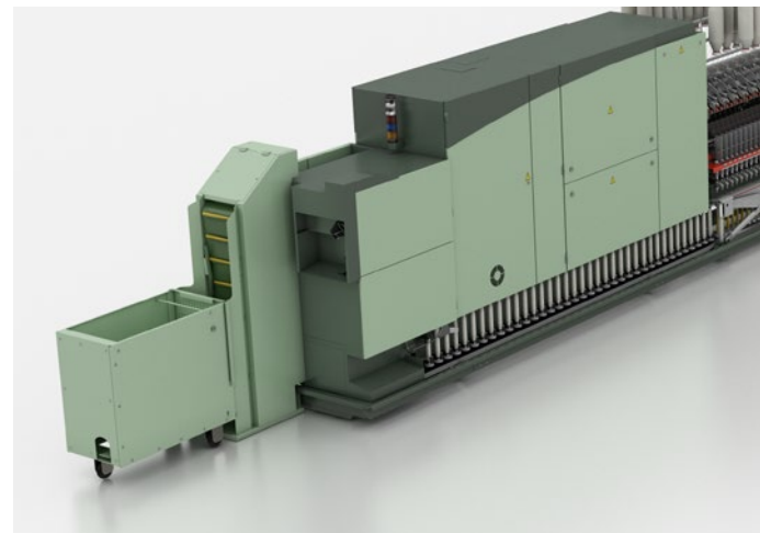
System WILDload: The tubes are picked up one after the other then aligned and fed to the tube loader ROBOload.
