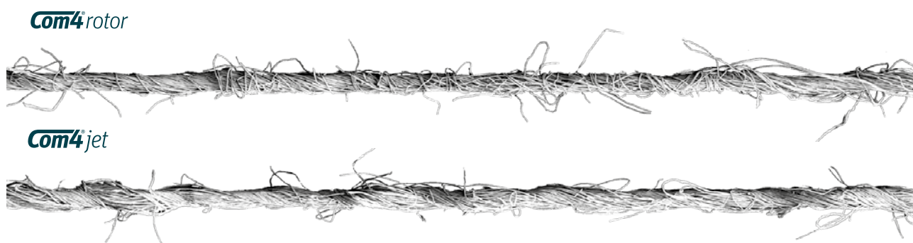
Fig. 12: Com4®rotor and Com4®jet yarn
