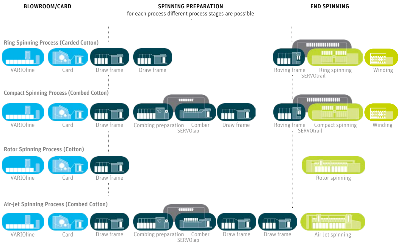
Fig. 18: Examples for complete manufacturing processes of the Com4® yarns
