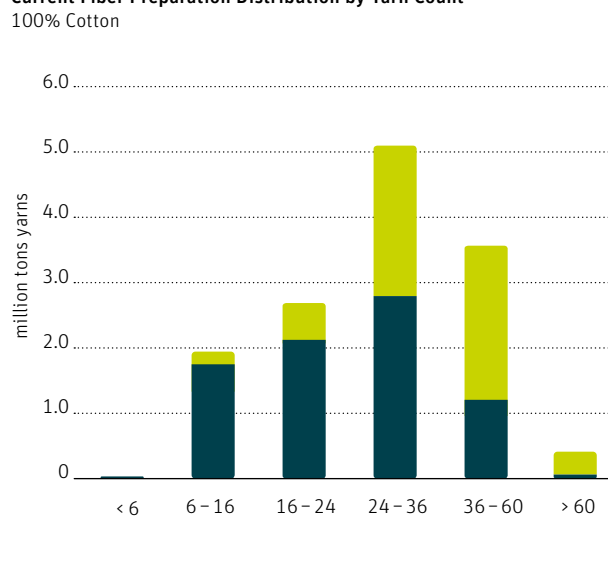
Fig. 32: Great differences in the quantities of combed feed material according to the spinning technology.
